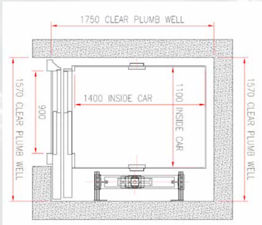
SINGLE ENTRY SHAFT PLAN
