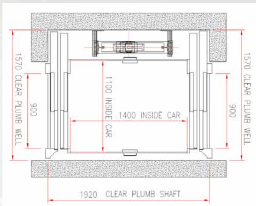
THRU CAR SHAFT PLAN
